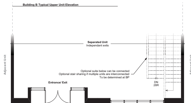
Building B Typical Upper Unit Plan
