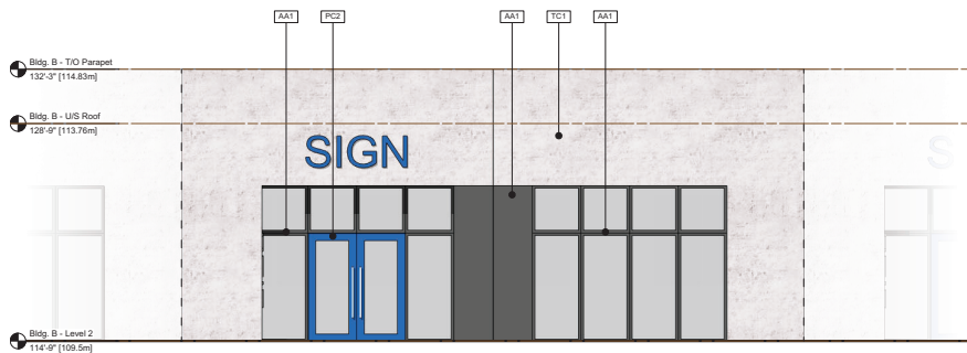
Building B Typical Upper Unit Elevation
